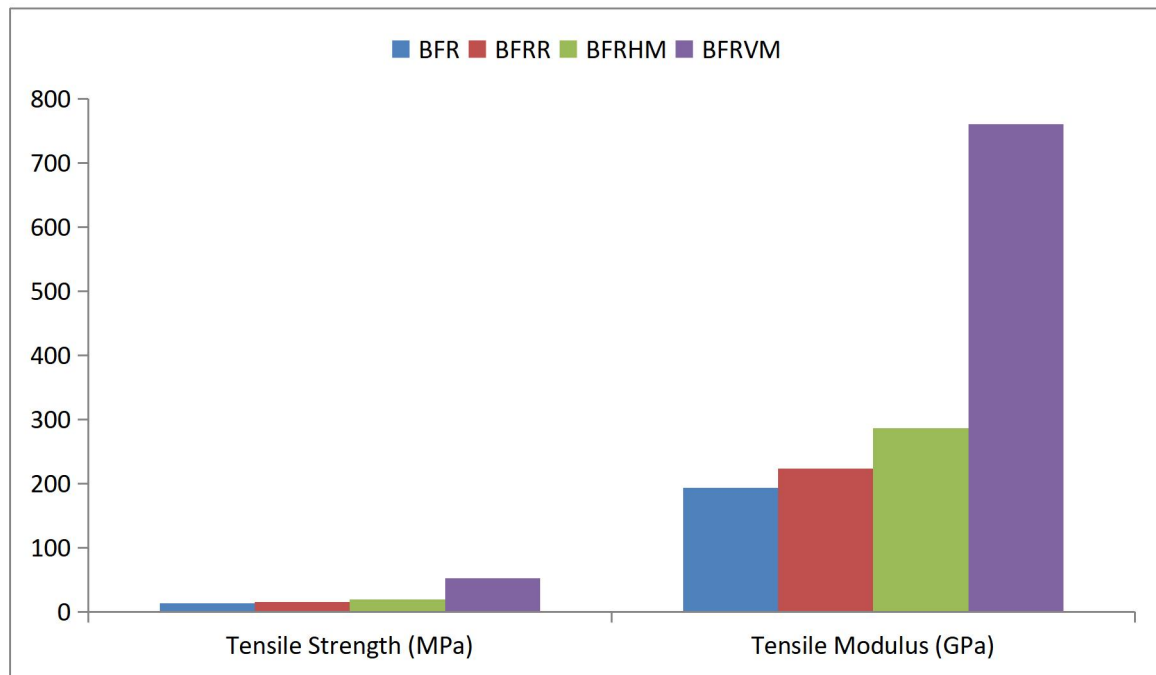
Figure 2(c): Tensile strength and tensile modulus of the four different composites
