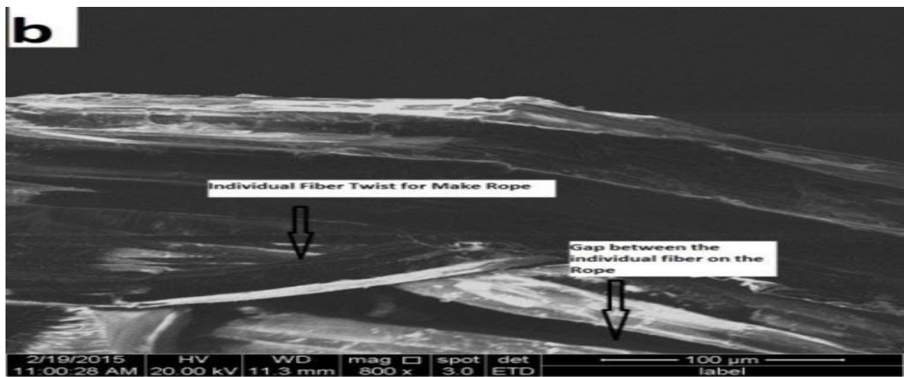
Figure 7(a - b): SEM images of impact-tested samples of banana fiber mat composites (a = 90x, b = 800x)
