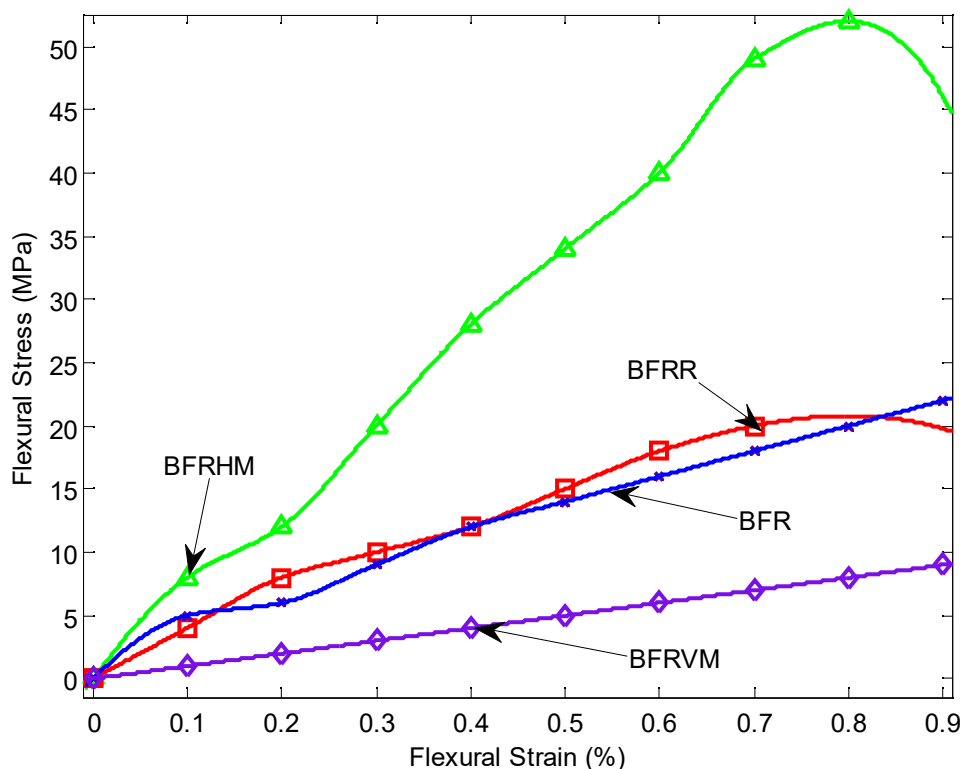
Figure 4(a): stress - strain curves of the four different composites
