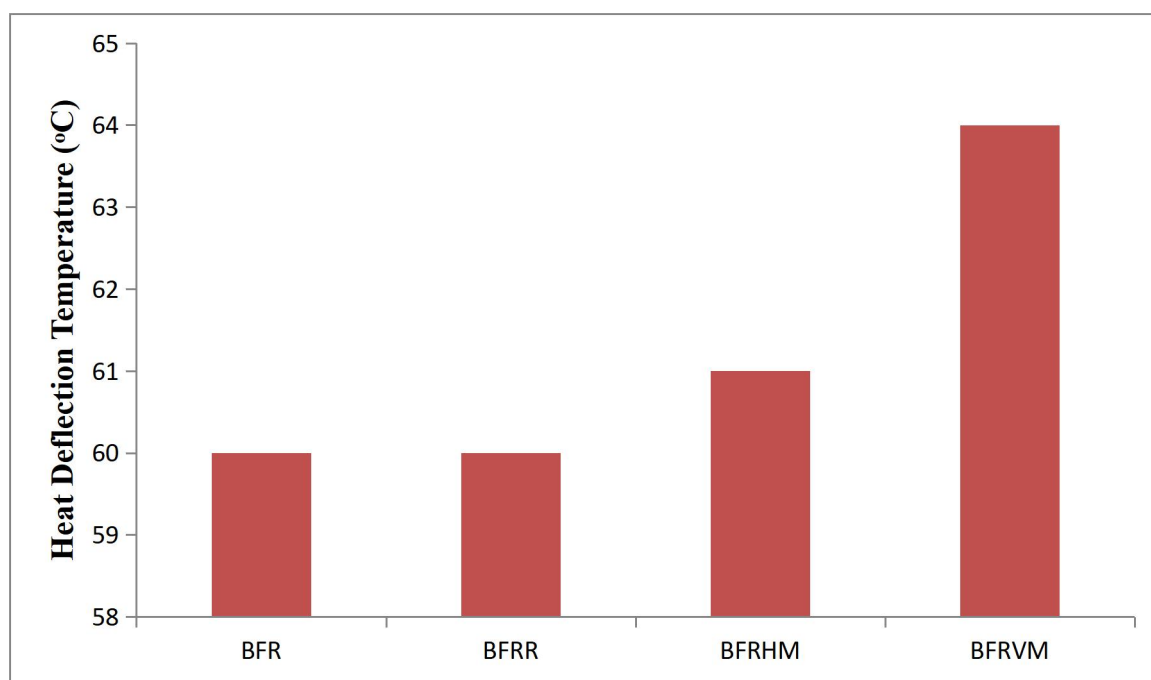
Figure 10: Heat deflection temperature test (HDT) for different forms of composites
