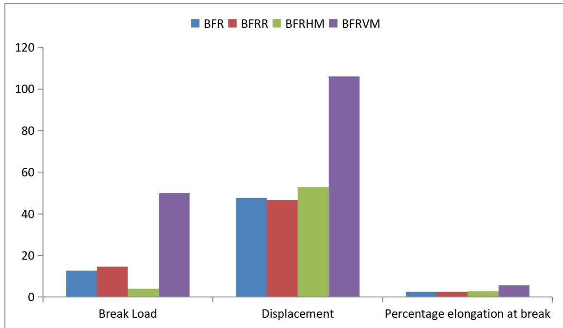
Figure 2(b): Break load, maximum displacement and percentage elongation at break of the four different composites
