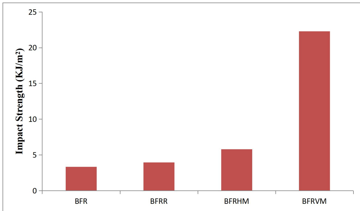
Figure 6: Impact strength for different fiber reinforced composites
