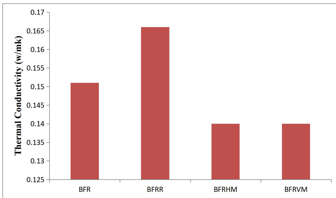
Figure 9: Thermal conductivity for different forms of composites
