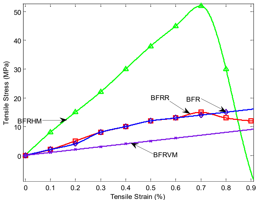
Figure 2(a): Stress - strain curves of the four different composites
