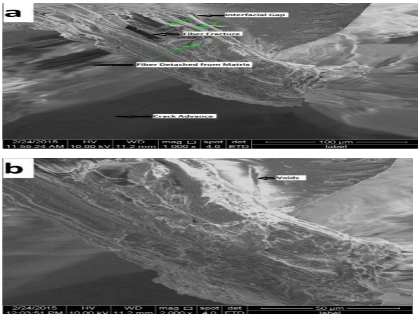
Figure 5(a - b): SEM images of flexure-tested samples of banana fiber mat composites (a = 1000x, b = 2000x)
