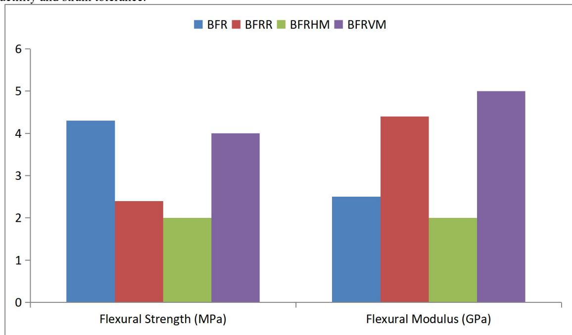
Figure 4(c): flexural strength and flexural modulus of the four different composites
