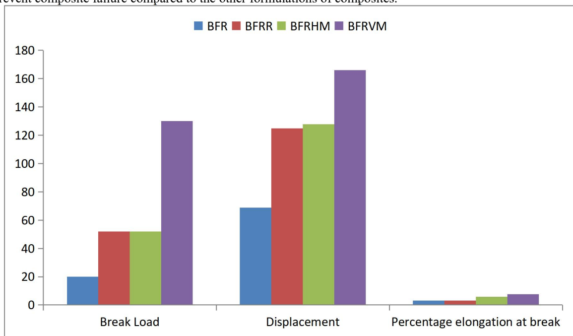
Figure 4(b): break load, maximum displacement and percentage elongation at break of the four different composites
